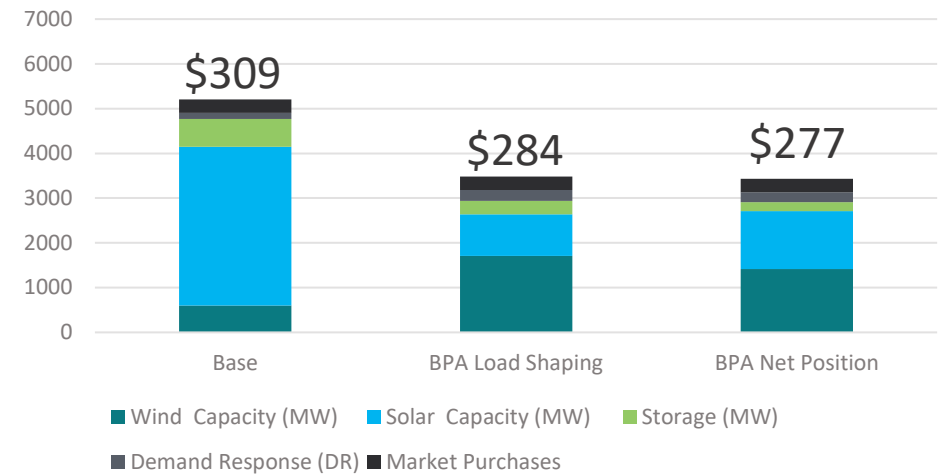
Replacement Capacity and Net Cost ($M/yr)
